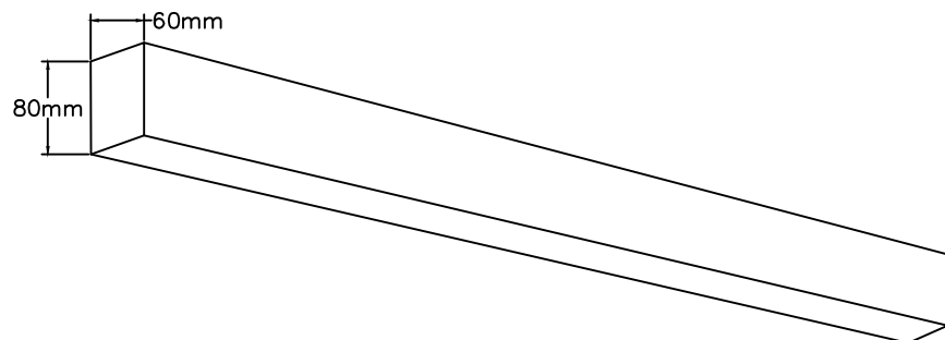
HL 6-1633A/860:860x60x80mm
